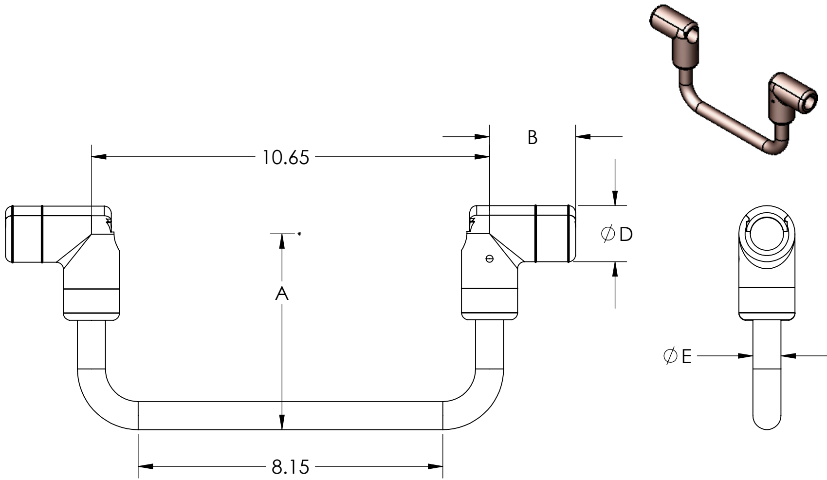
FIGURE 1: STANDARD STIRRUP ROD LENGTH
